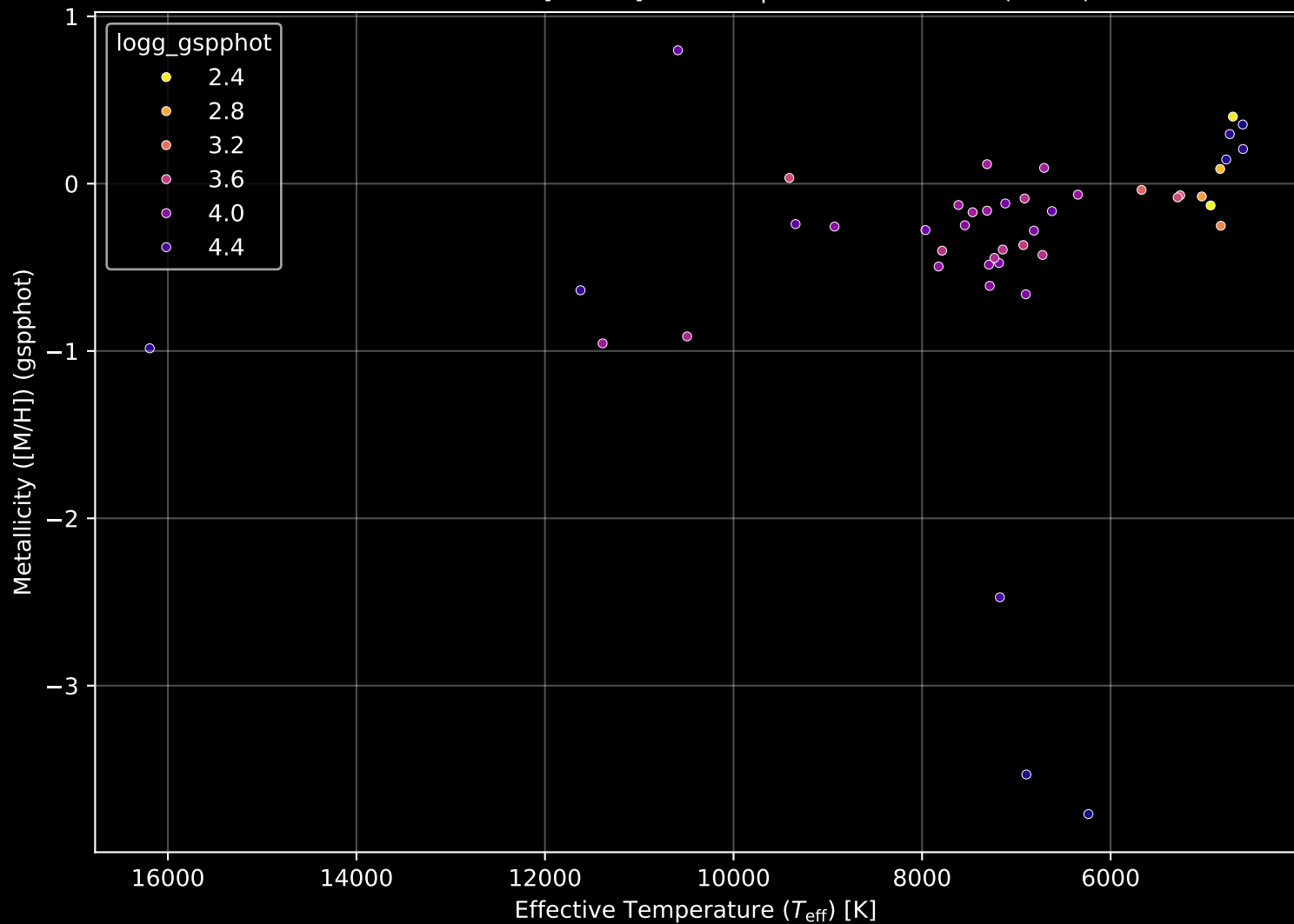
APOGEE DR17 Field: [ANDR2] Stellar Population Parameters (n= 45)
