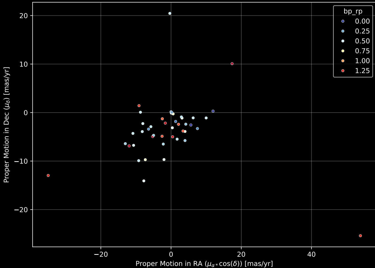
APOGEE DR17 Field: [ANDR2] Proper Motion Diagram (n= 45)
