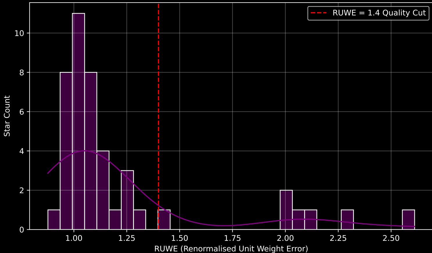
GAPOGEE DR17 Field [ANDR2] RUWE Distribution (n= 44)
