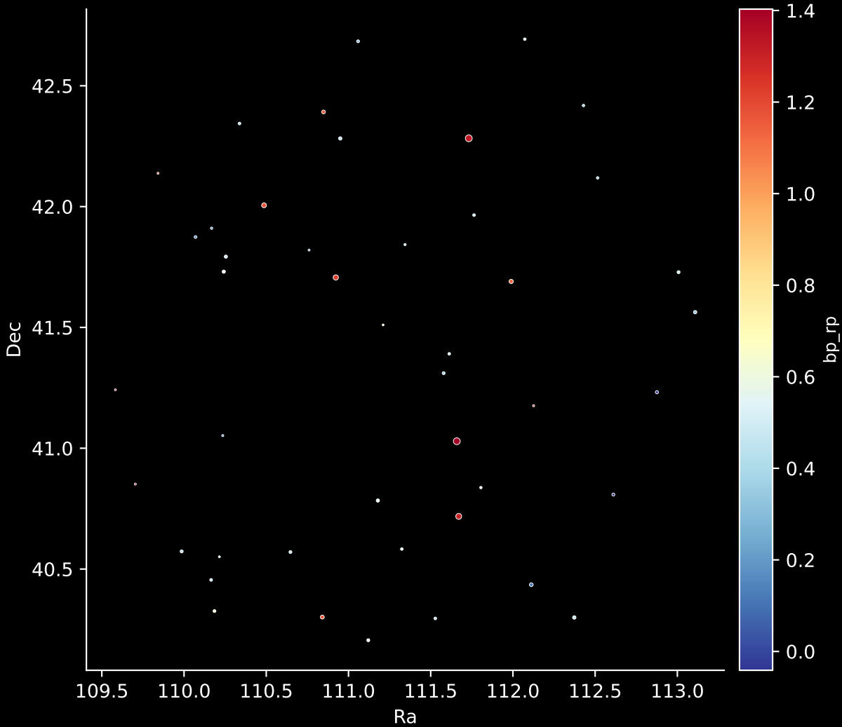
APOGEE DR17 Field: [ANDR2] Stars: 45
