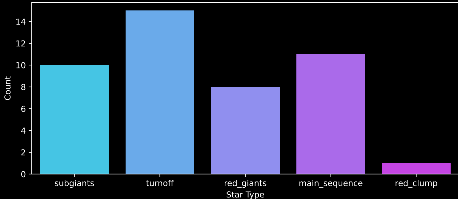
APOGEE DR17 Field: [ANDR2] Count plot of Star Type
