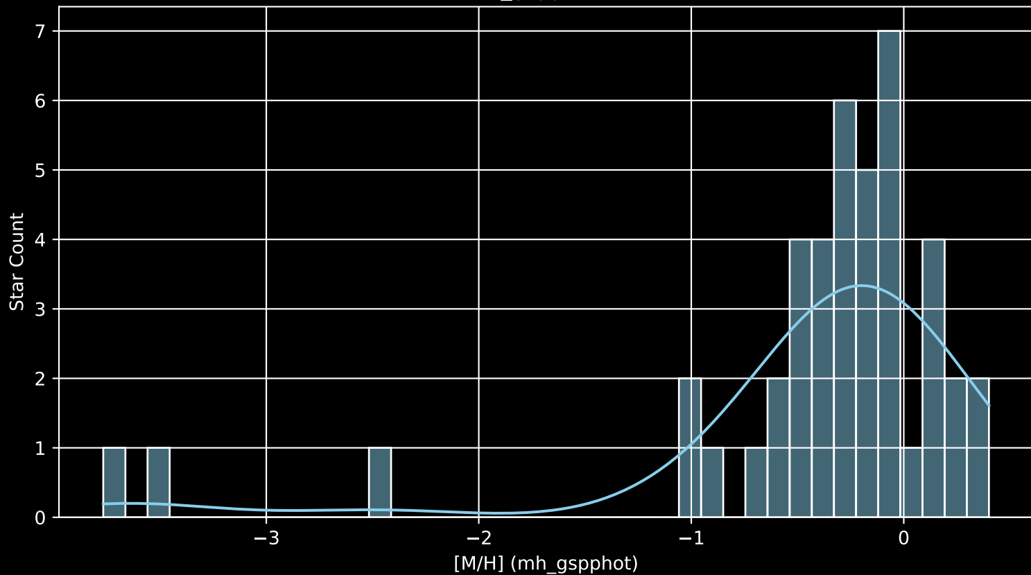
APOGEE DR17 Field: [ANDR2 [M/H] (mh_gspphot) (n= 44)
