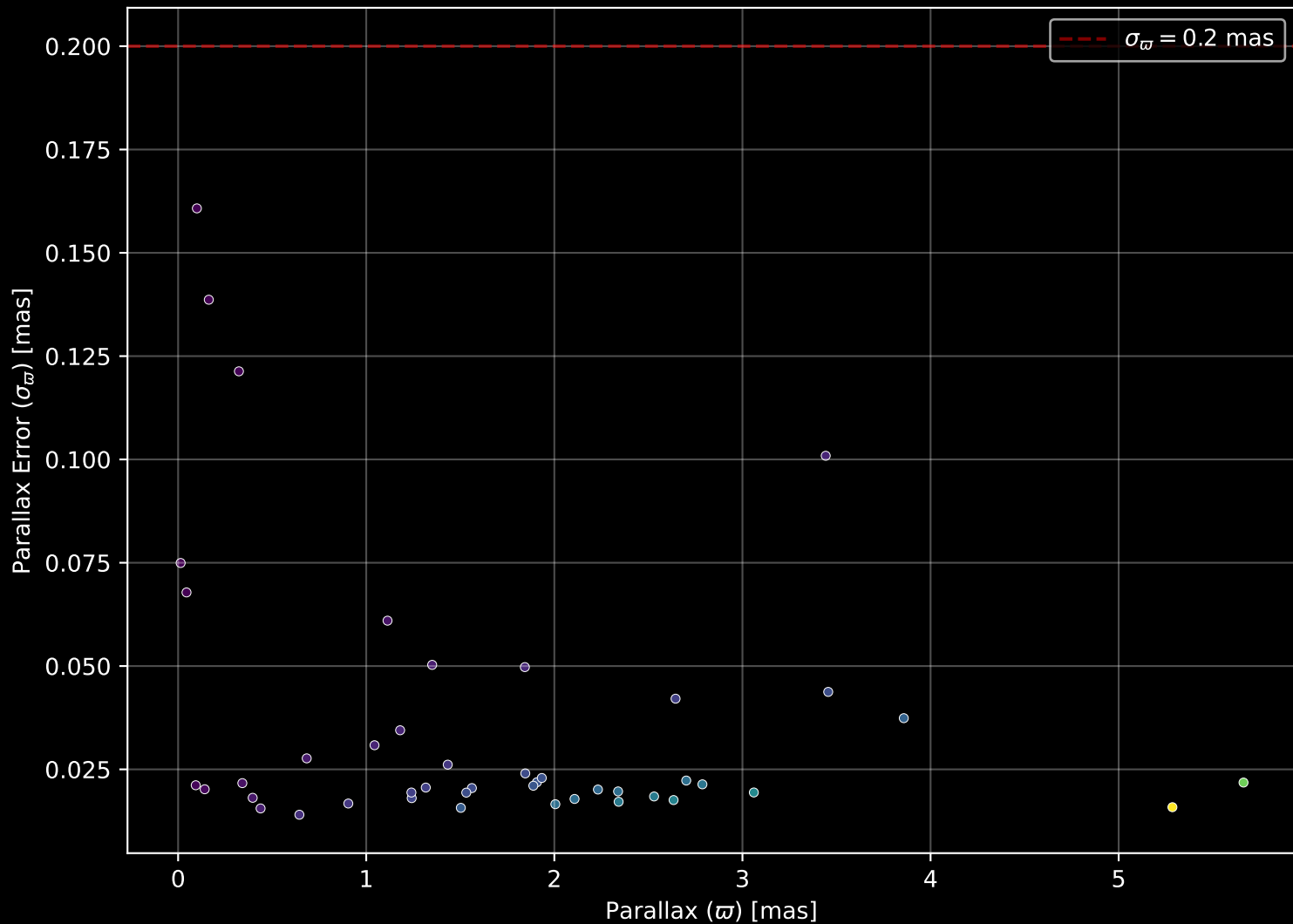
APOGEE DR17 Field: [ANDR2] Parallax Quality (n= 45)
